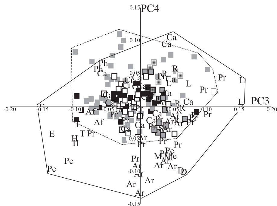
Figure 4 Principal components (PC)3 and 4 for the 'maximum taxa' dataset. Symbols as in Figure 2.
